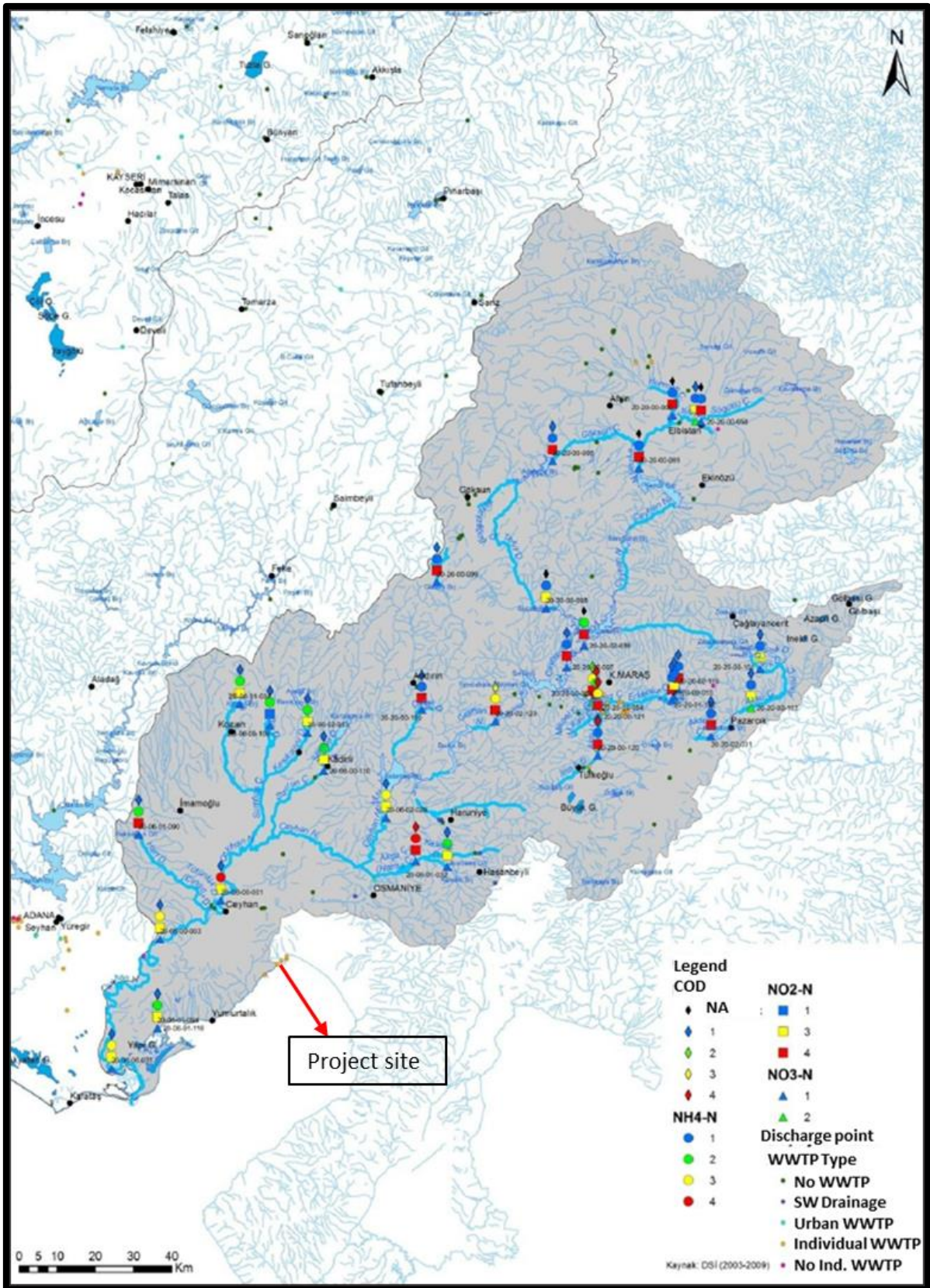
Figure 1. Water quality classes (COD, NH4-N, NO2-N, NO3-N)
